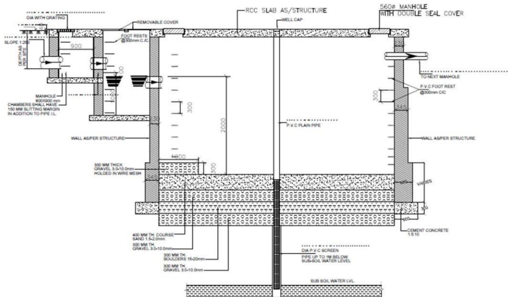
SECTION-XX DETAIL OF RECHARGE WELL 6.00mx2.5m
